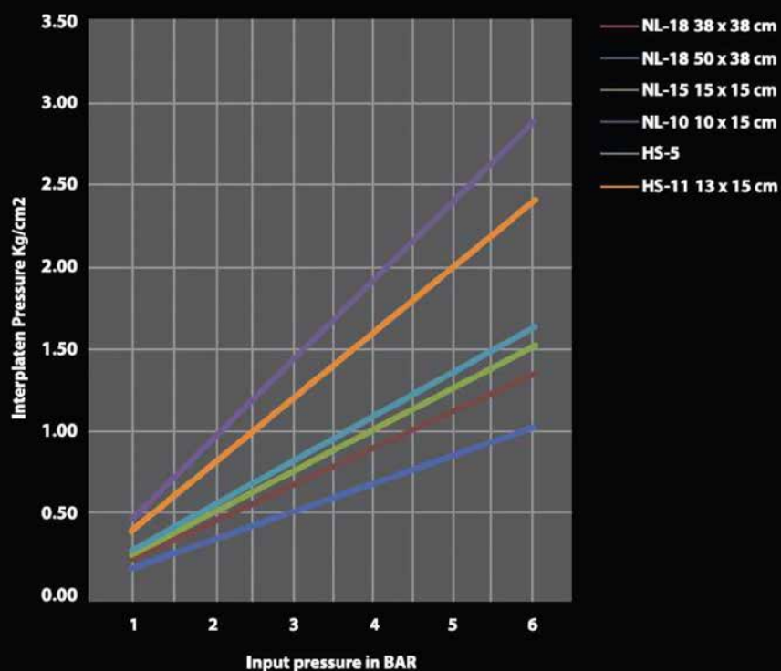
heat seal press interplaten pressure
